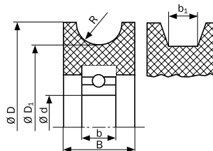
Execution without axle (diagrammatic sketch)
